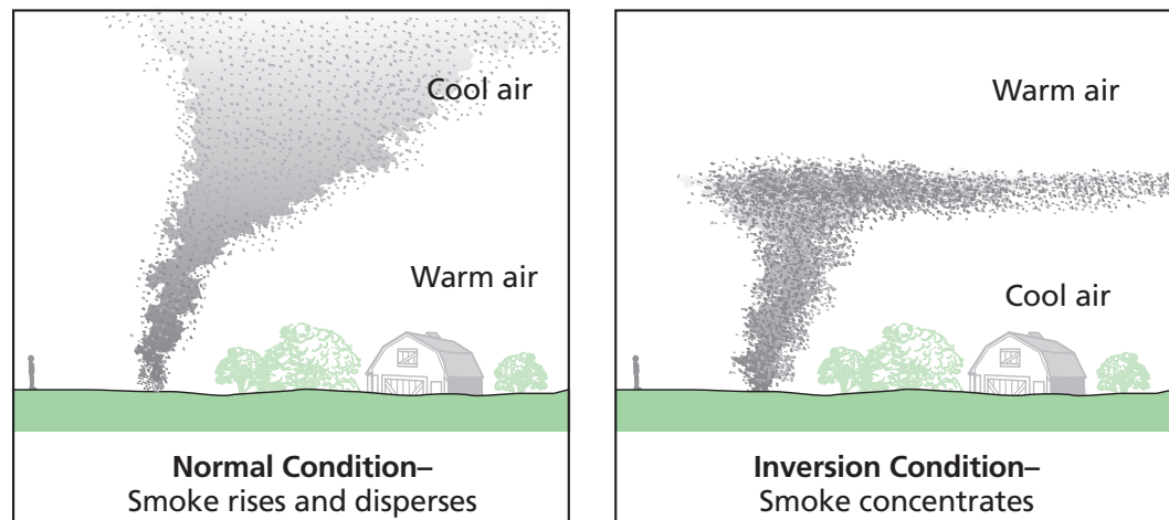
Figure 7.3 Dispersion of smoke particles under normal and inversion conditions.
