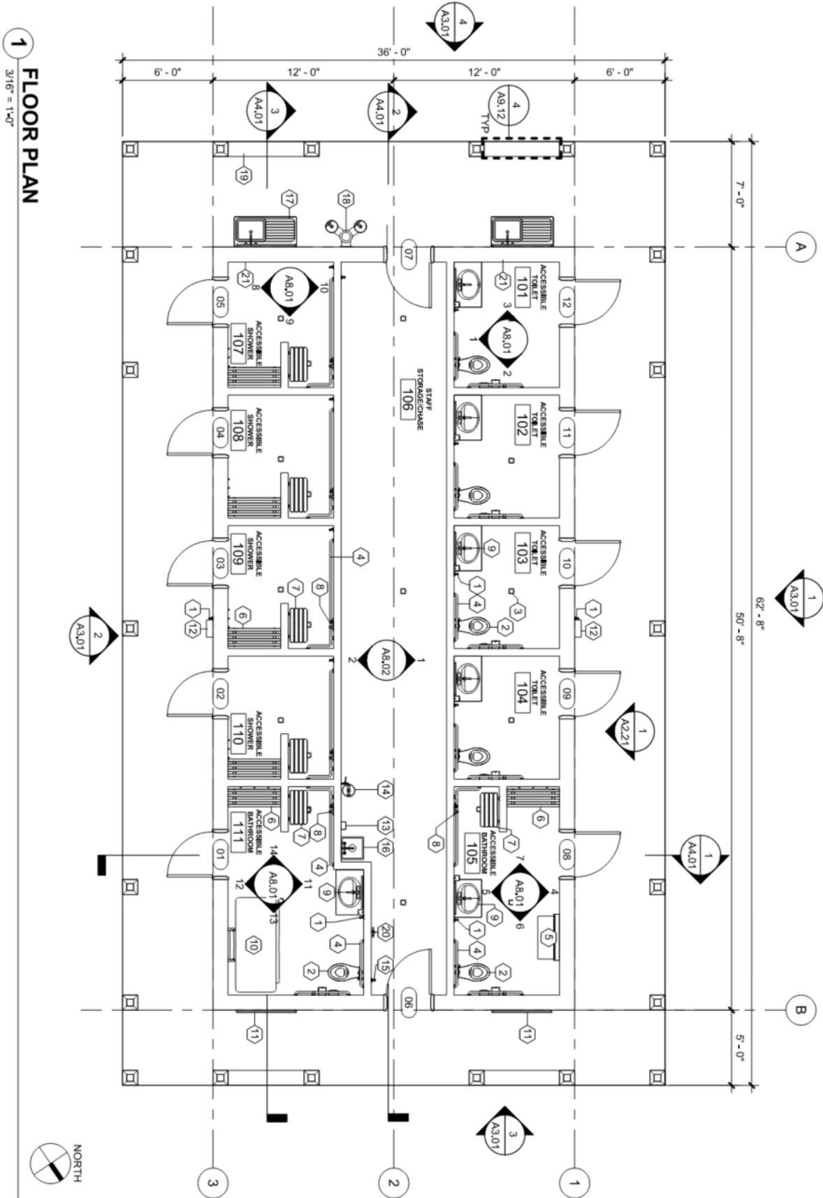
Figure C – Proposed Building Floor Plan
