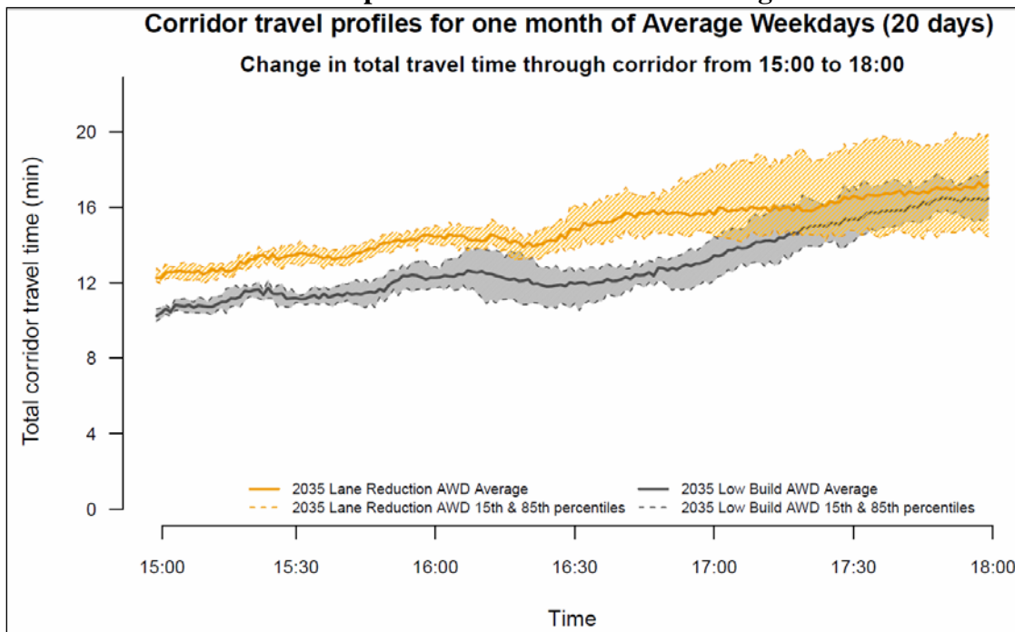
Exhibit 8-20 DTA MOE Sample 2 – Travel Time Profile along a Corridor
