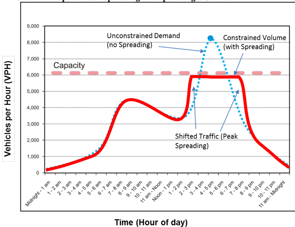
Exhibit 8-22 Temporal Peak Spreading Example along a Corridor
