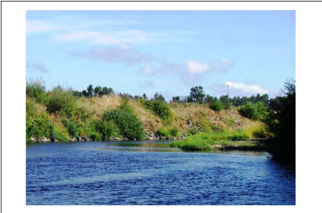
Figure 6-9. More obscure riprap along the Calapooia River near Albany, Oregon. Herrera Environmental Consultants.
