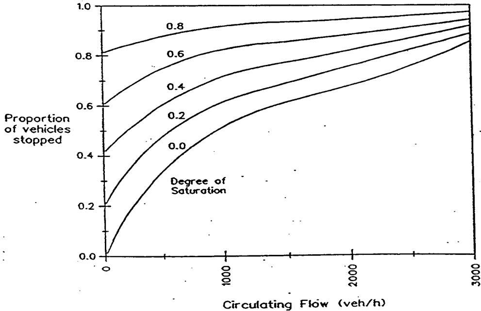
Figure 6.7: Proportion of Vehicles Stopped on a Multi-Lane Entry Roundabout ( Austrad 1993 )
