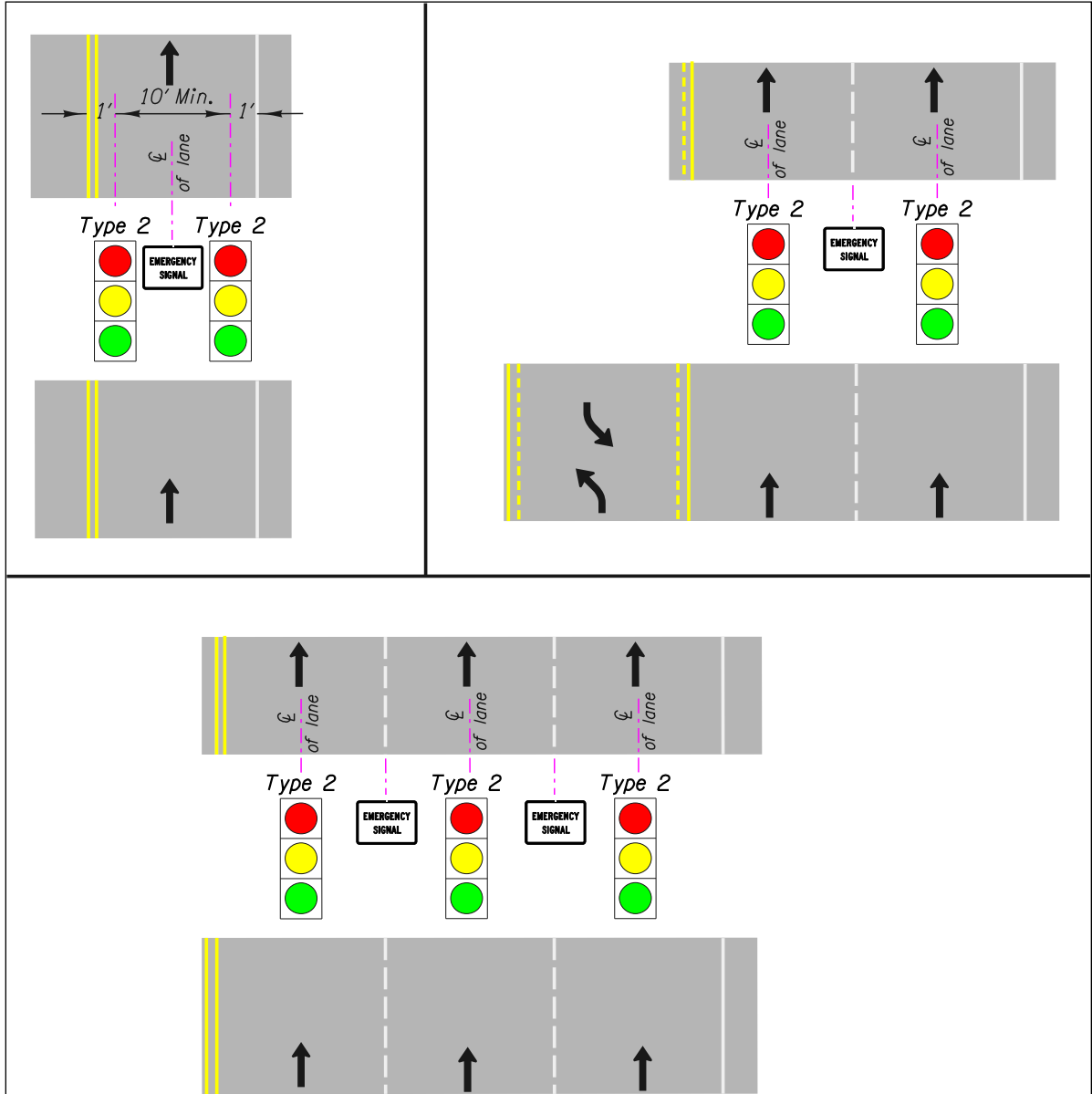
Figure 17-2 | Signal Head Layout for Mid-Block Fire Signal
