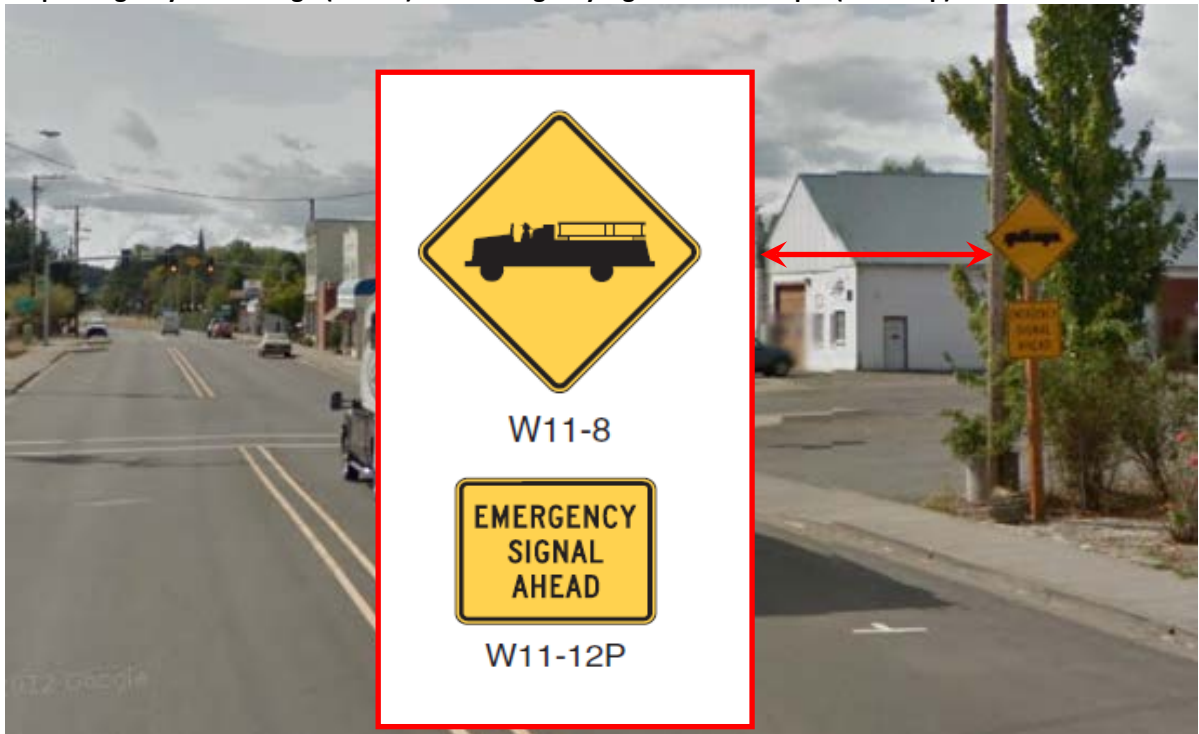
Figure 17-6 | Emergency Vehicle Sign (W11-8) with Emergency Signal Ahead Plaque (W11-12p)
