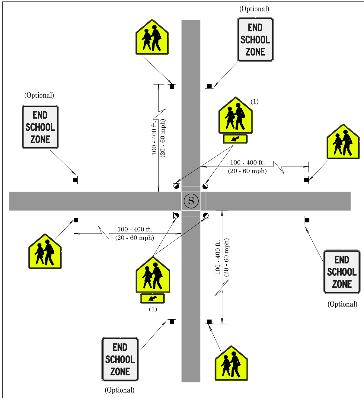
Figure 197: School Crosswalk Away From School at Signalized Intersection (Optional)
