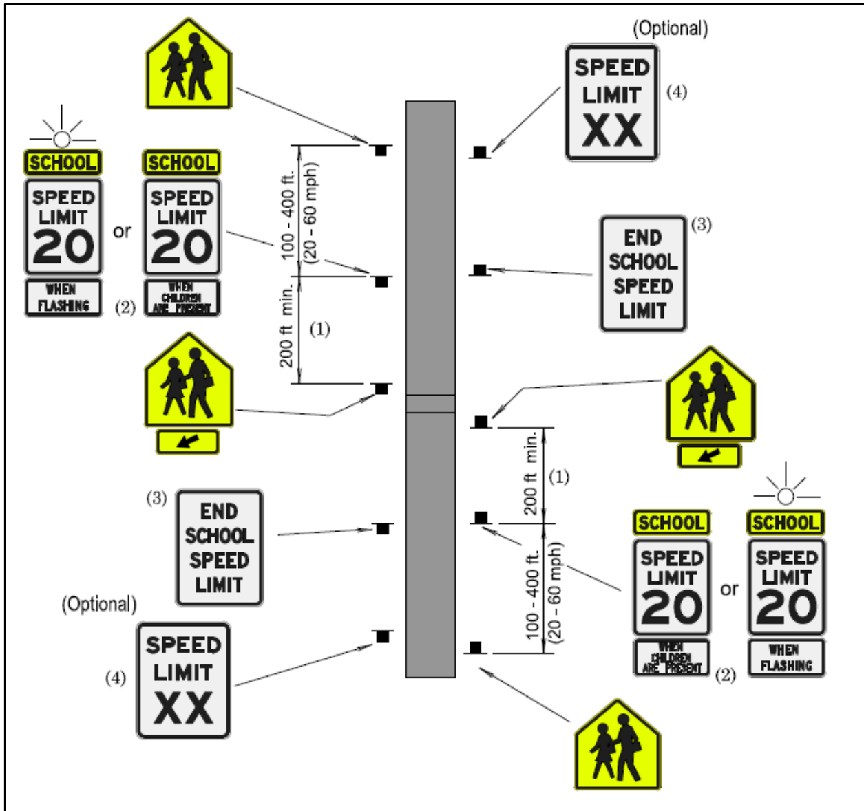
Figure 196: Condition "B" School Crosswalk Not Adjacent To School Grounds
