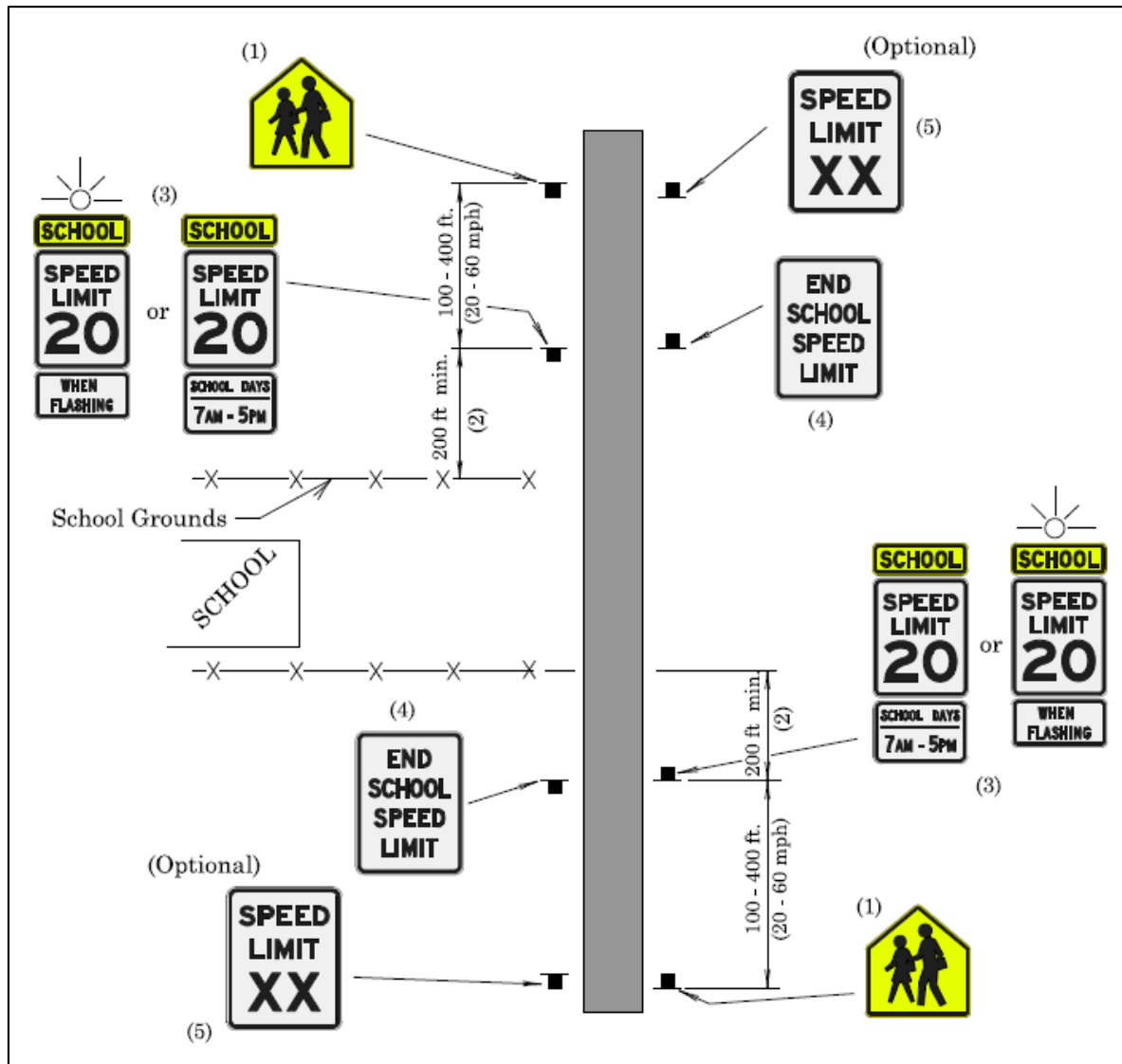
Figure 194: Condition "A" Layout without School Crosswalk
