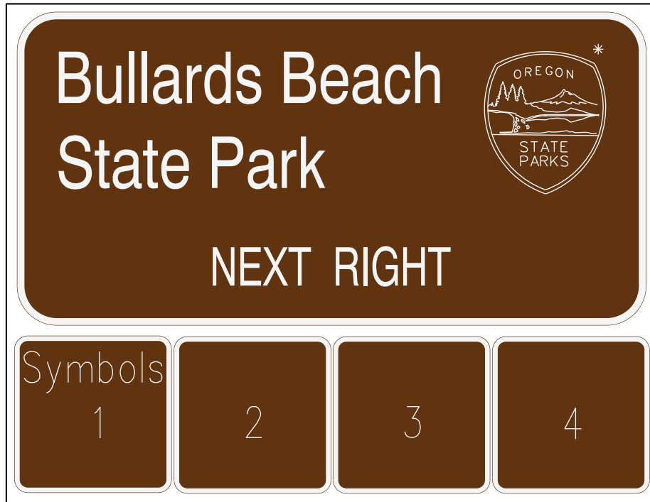
Figure 117: Sign D-435 Detail
