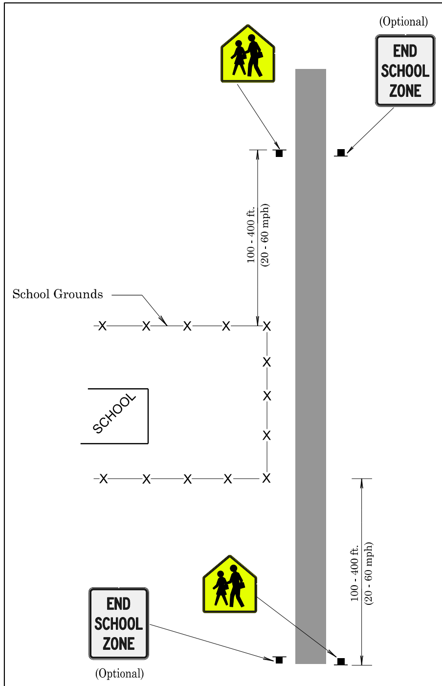
Figure 198: School Building Away From Highway or School Grounds Fenced (Optional)
