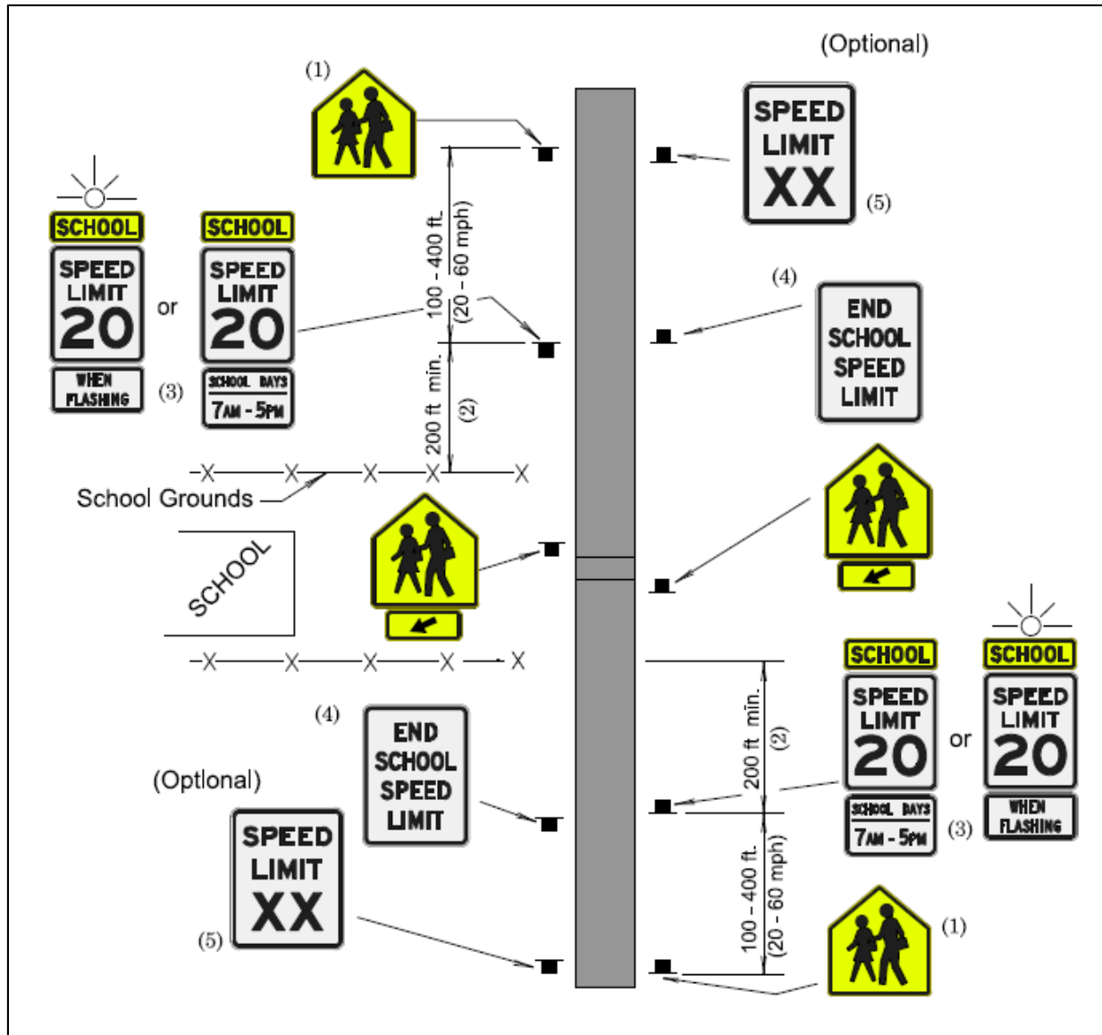
Figure 195: Condition "A" Layout with School Crosswalk
