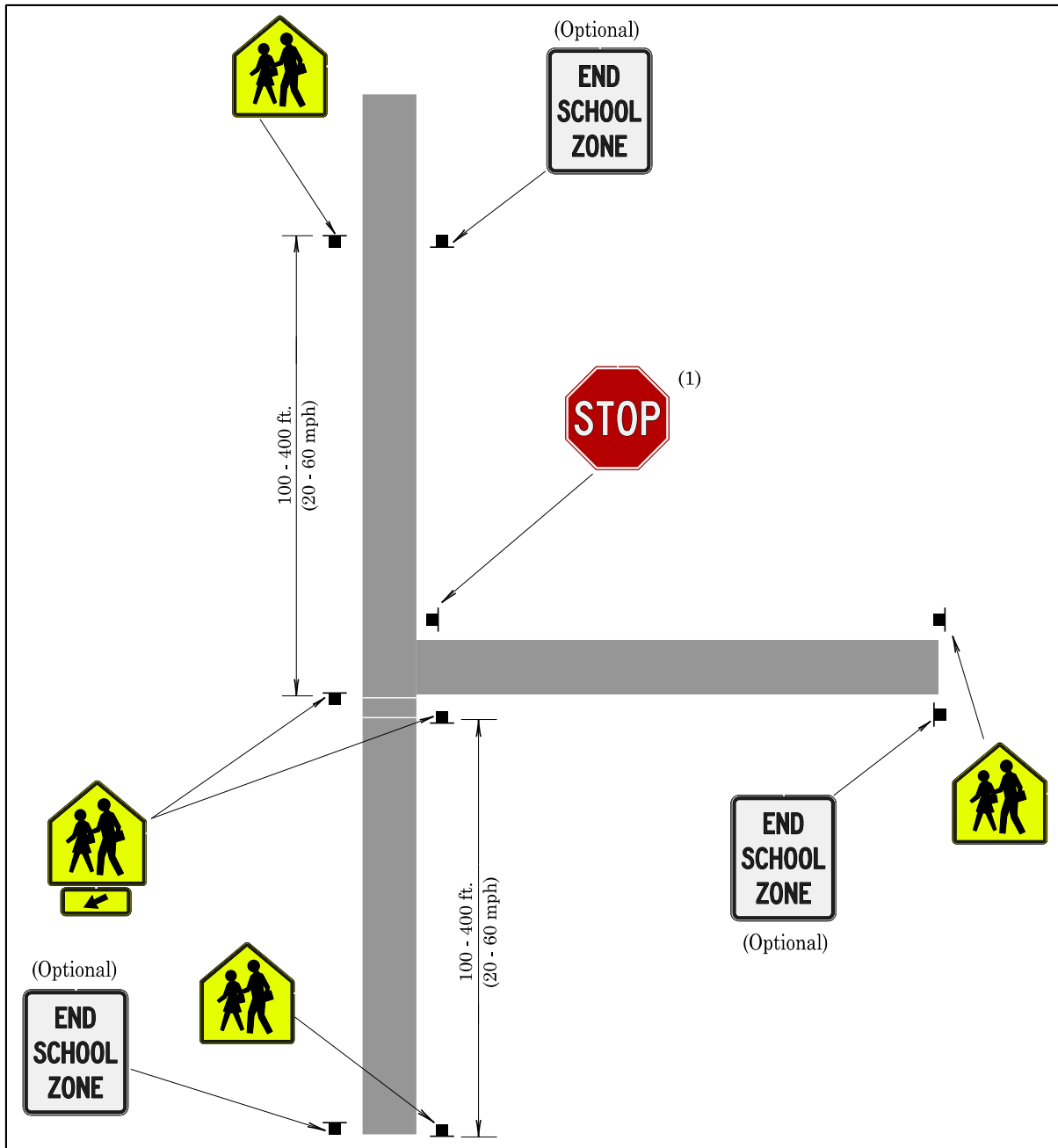
Figure 199: School Crosswalk Away From School (Optional)
