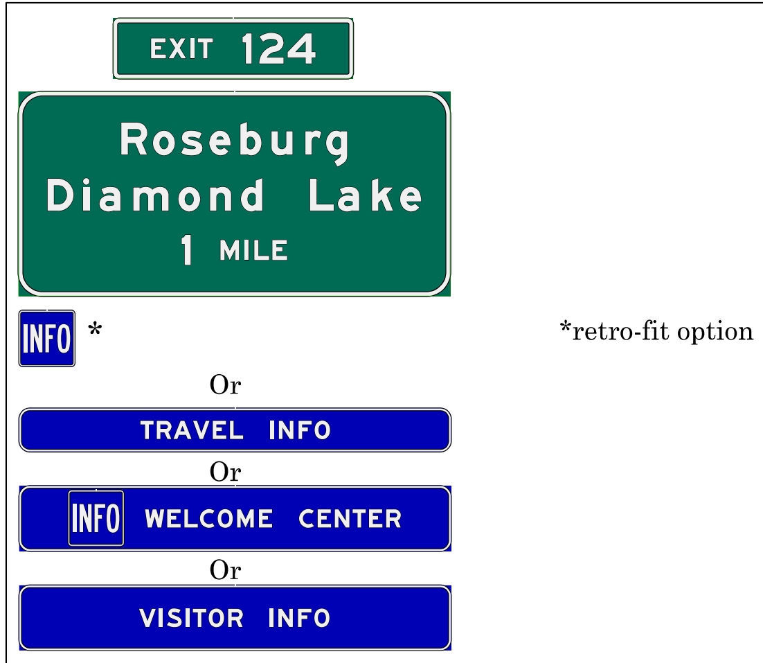
Figure 101: Typical Freeway sign for Travel Info. Center in rest area
