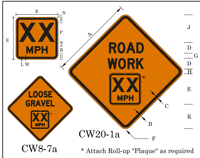
Figure 173: Signs CW20-1a & CW8-7a (ROAD WORK (LOOSE GRAVEL) XX MPH) Detail
