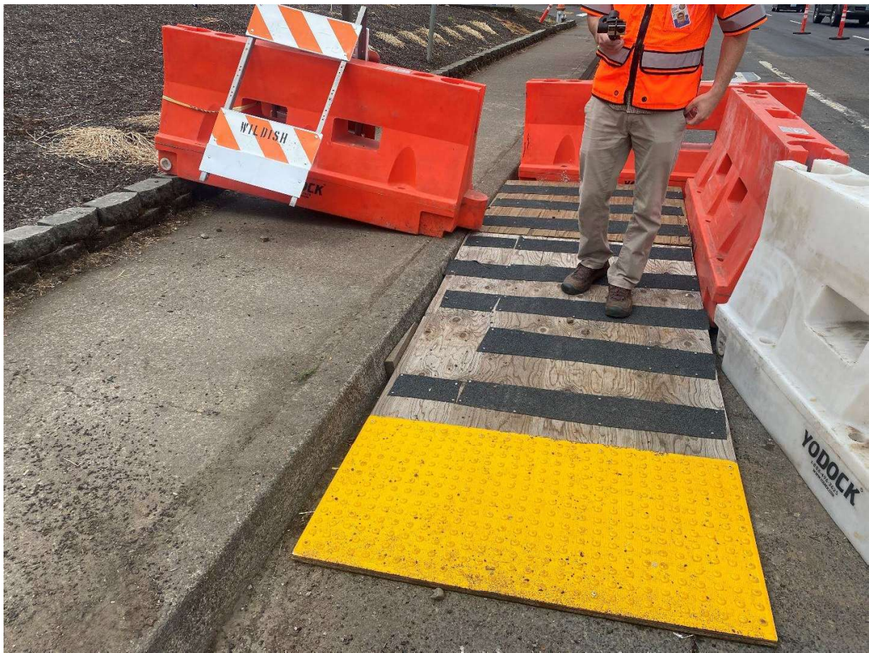
Temporary pedestrian ramp with a detectable warning surface.
