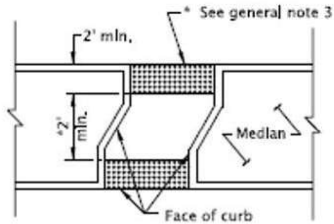
CUT-THROUGH (Asph. conc. surface shown)
