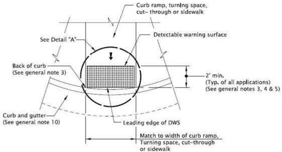
DETECTABLE WARNING SURFACE DETAIL
