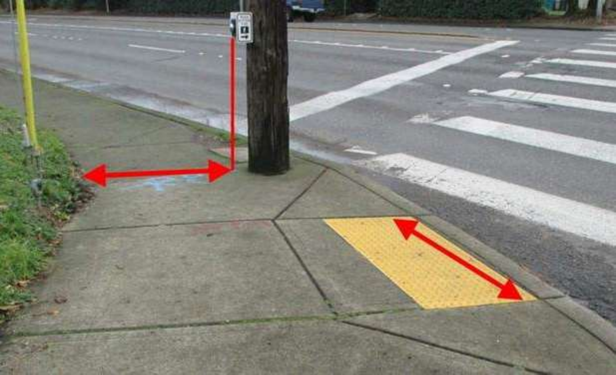
Example of Clear Width Measurement Locations
