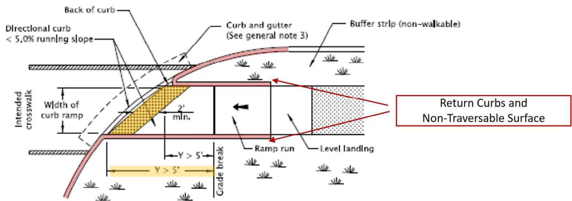
CURB RAMP CROSSING GRADE BREAK > 5 FT. FROM BACK OF CURB
