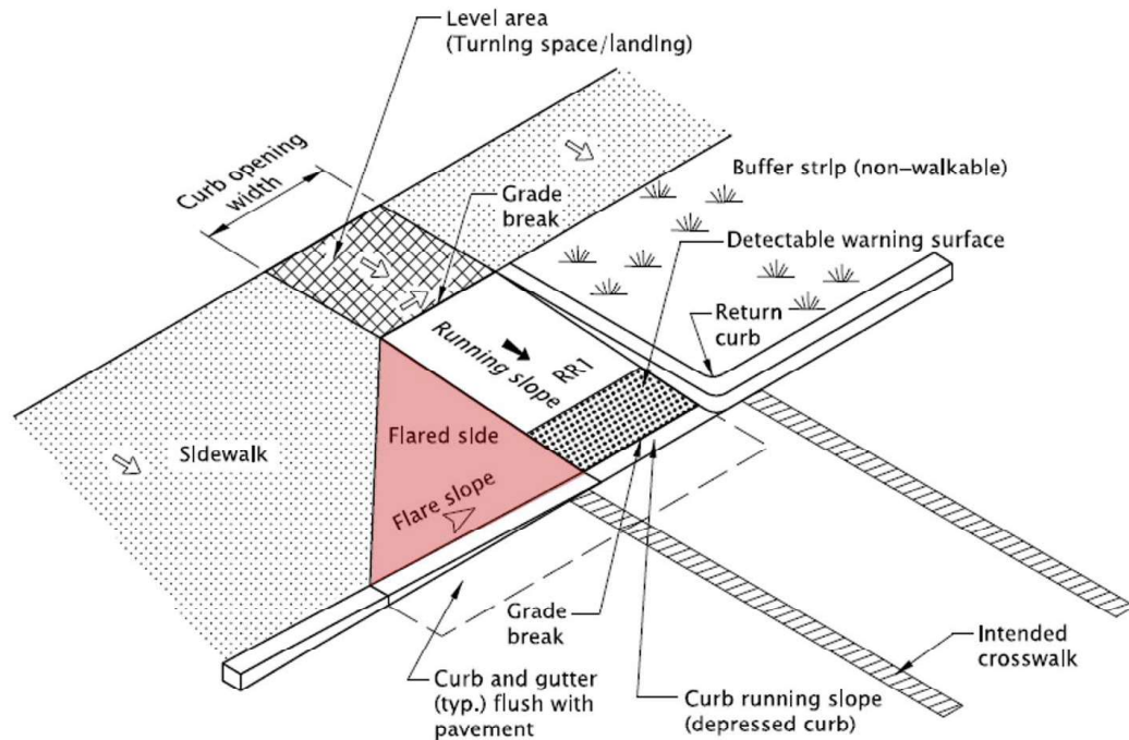
Flared Side Treatment
