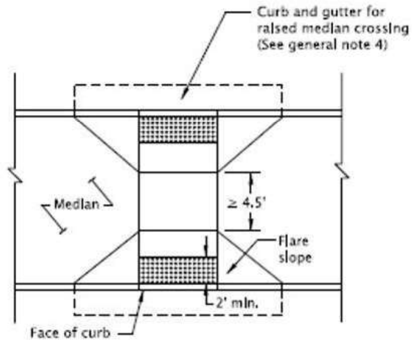
RAISED MEDIAN (P.C. conc. surface shown)
