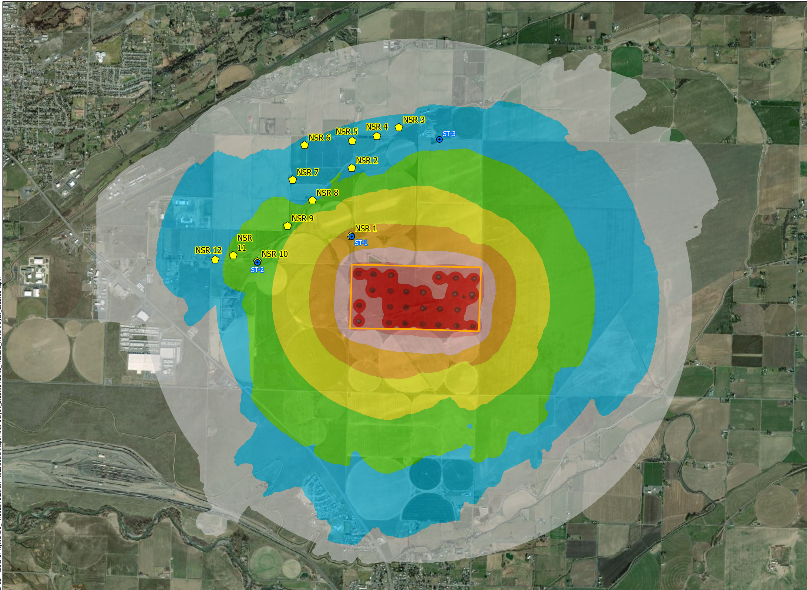
Figure Y-1 Operational Received Sound Levels (Distributed Battery Storage)
