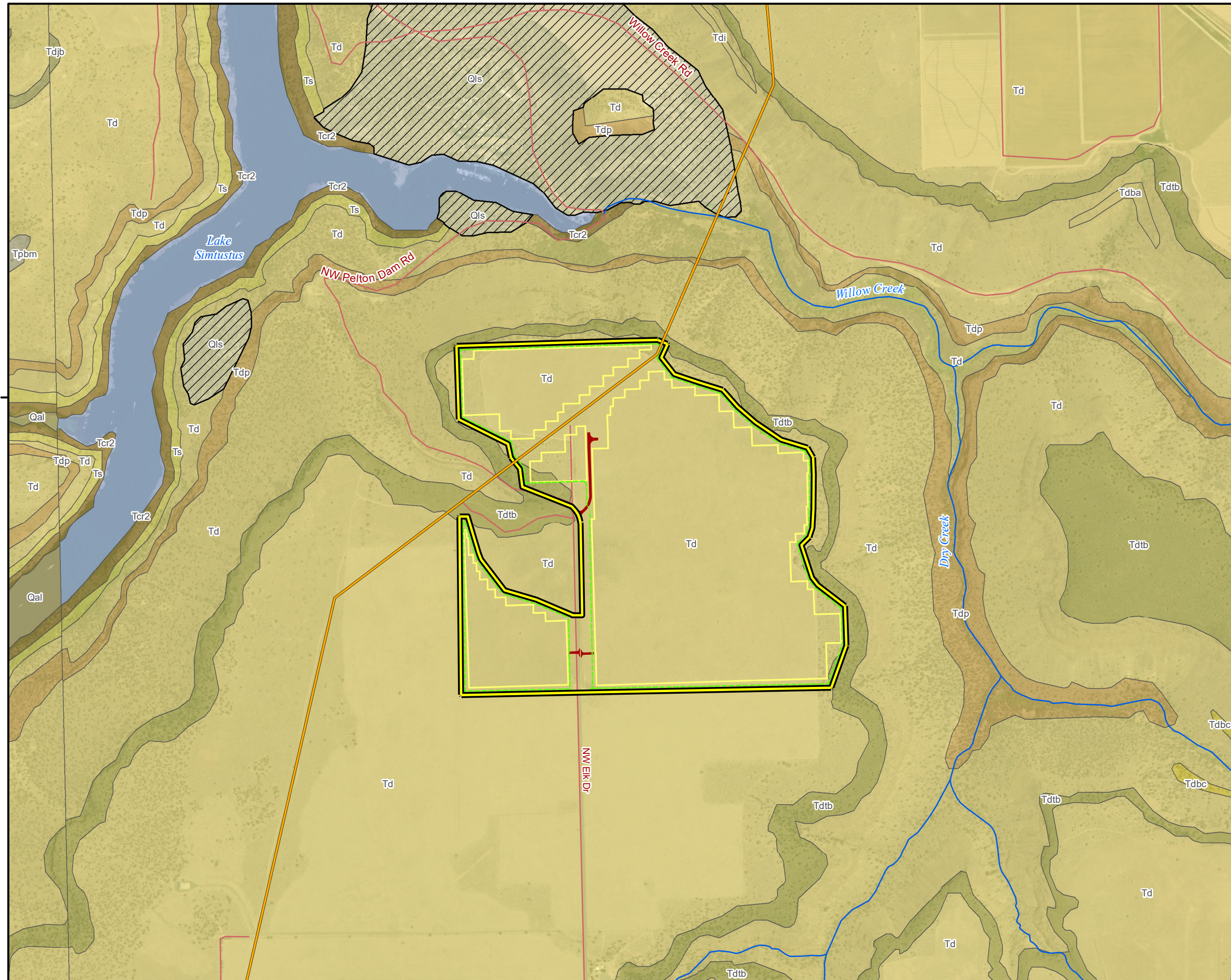
Figure H-1 Geology Map Application for Site Certificate Madras Solar Energy Facility Jefferson County, OR
