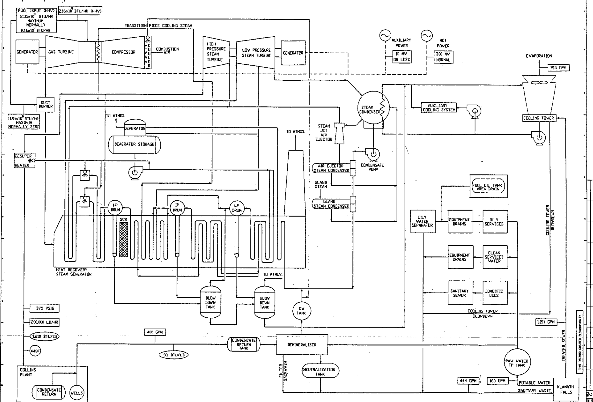
PROCESS FLOW DIAGRAM FIGURE B-1
