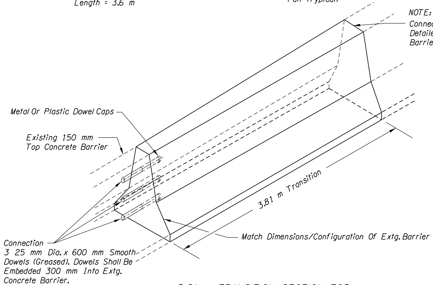
3.81 m TRANSITION SECTION FOR MEDIAN BARRIER OR SHOULDER BARRIER (CAST IN PLACE)
